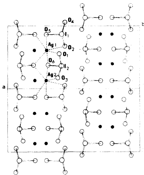
FIG. 1. Projection ( a, b ) de la structure \text{AgIO}_3 .
